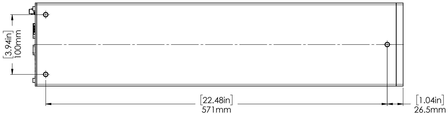
Bottom View
