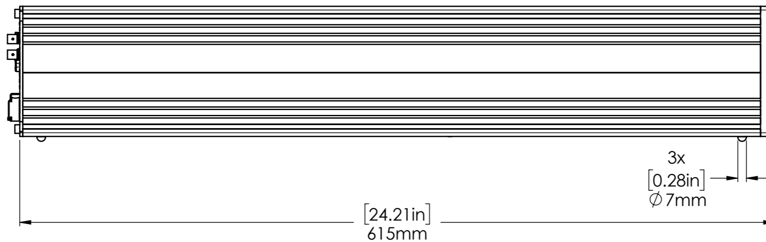
Top View
