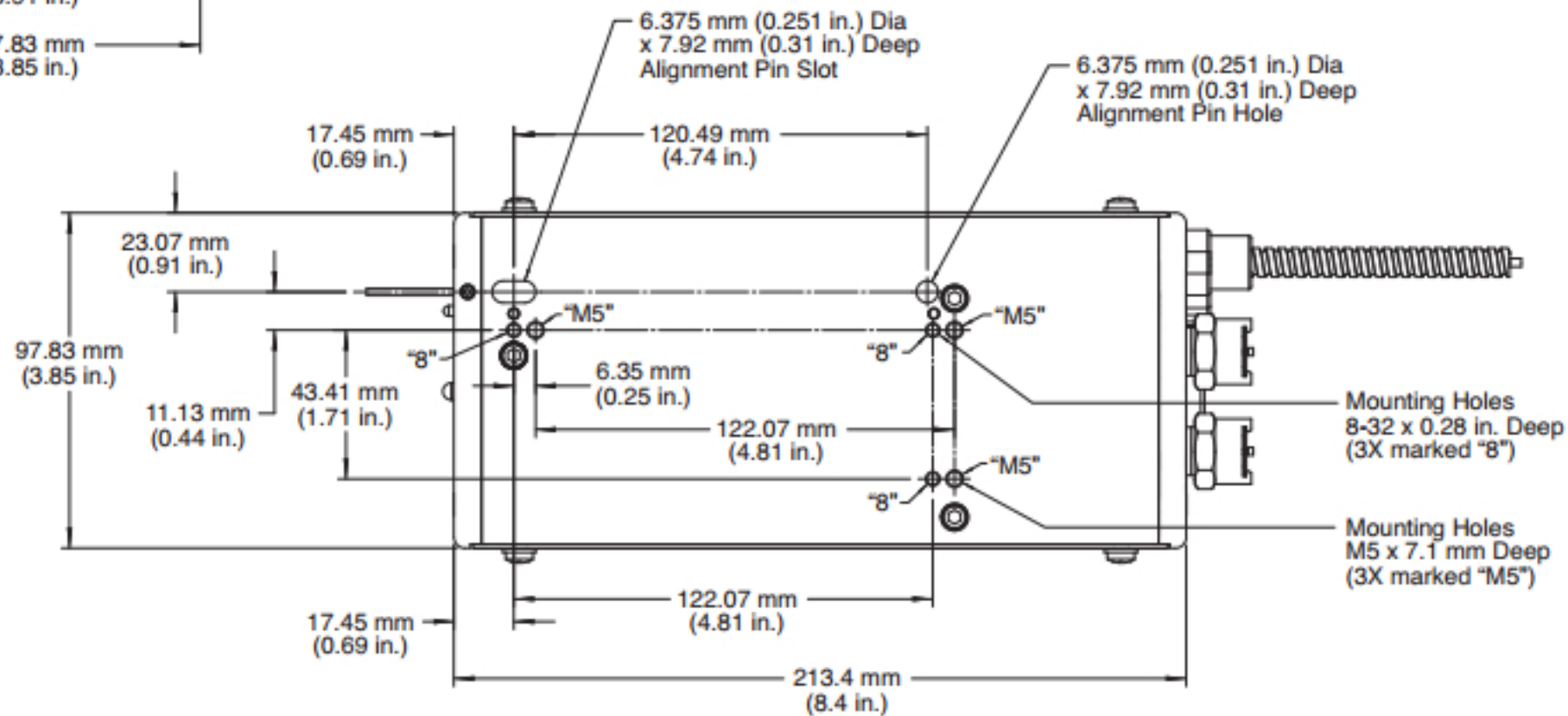
Bottom View
