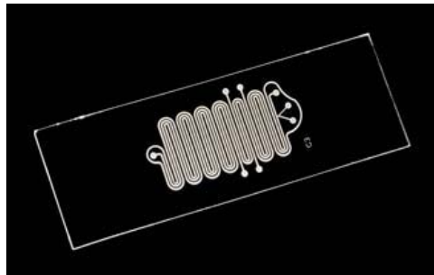
Figure 1. Picosecond lasers provide a flexible and versatile method of creating complex grooves, holes, and wells in various materials, including in glass microscope slides.
