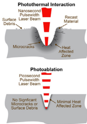
Figure 2. By removing material partially through photoablation, picosecond lasers produce higher-quality holes than traditional laser techniques.
