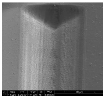
Figure 4. A microfluidic channel machined in FEP using a 355-nm picosecond laser.
